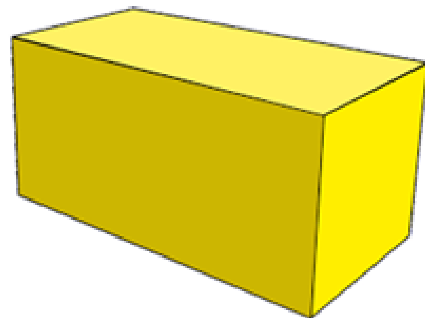
Cuboid
