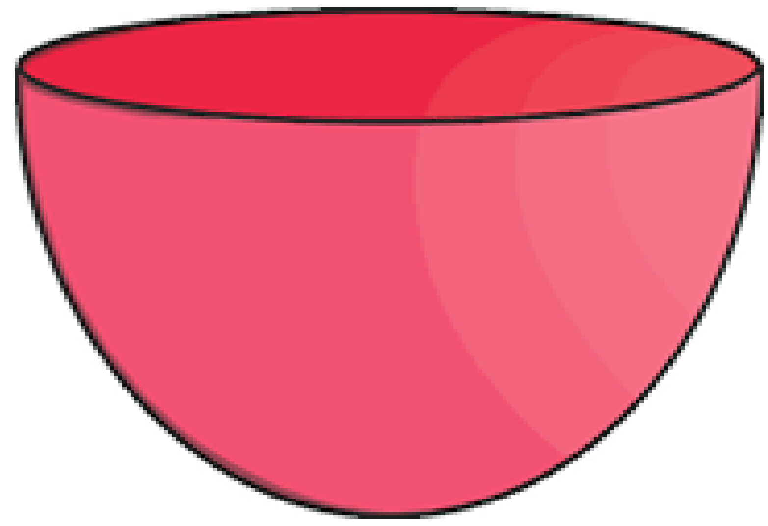
Hemisphere
