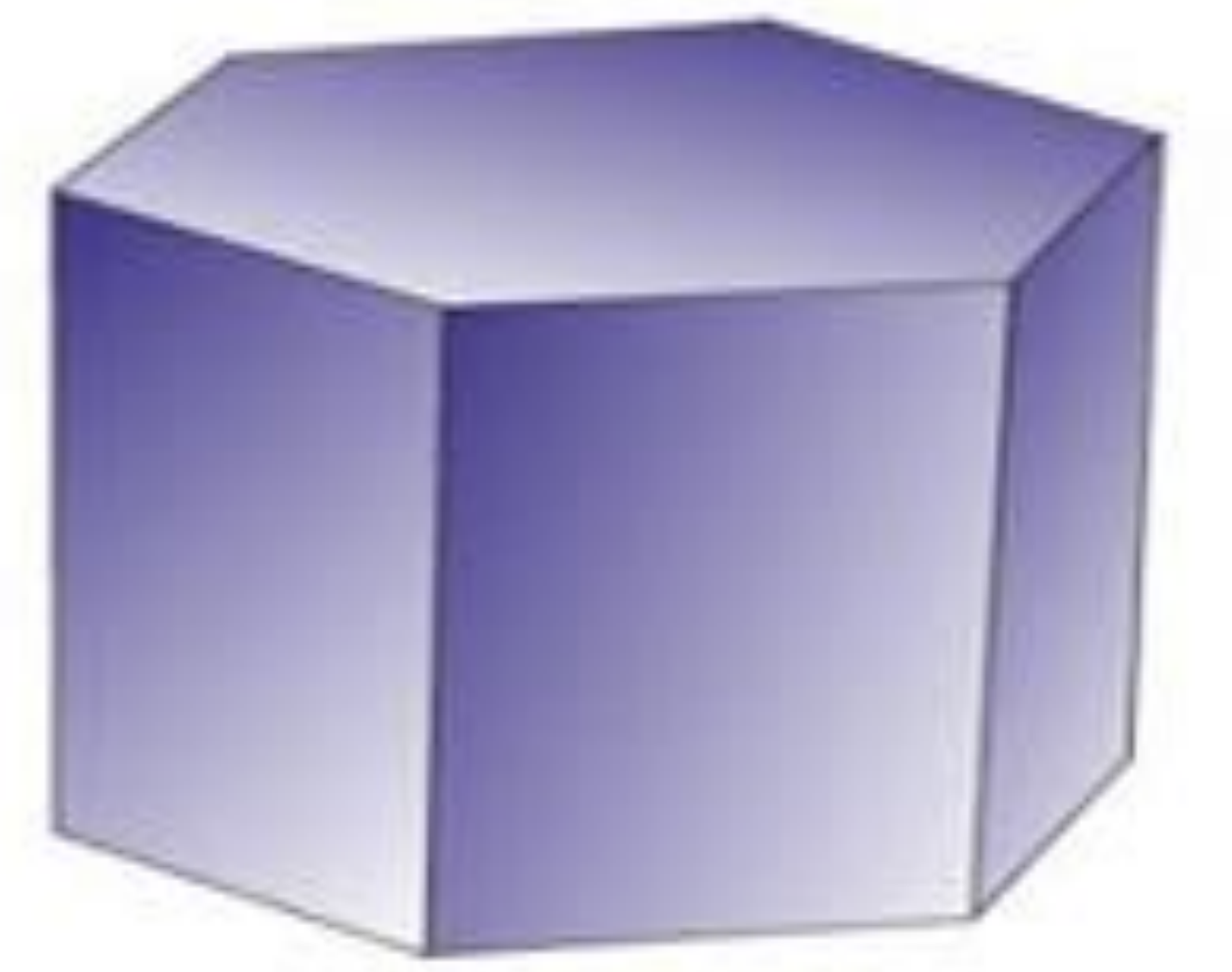
Hexagonal prism
