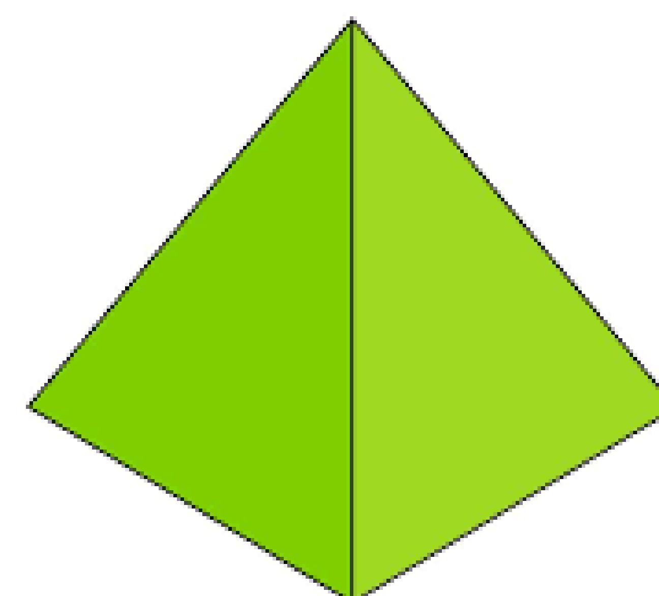
Square Pyramid
