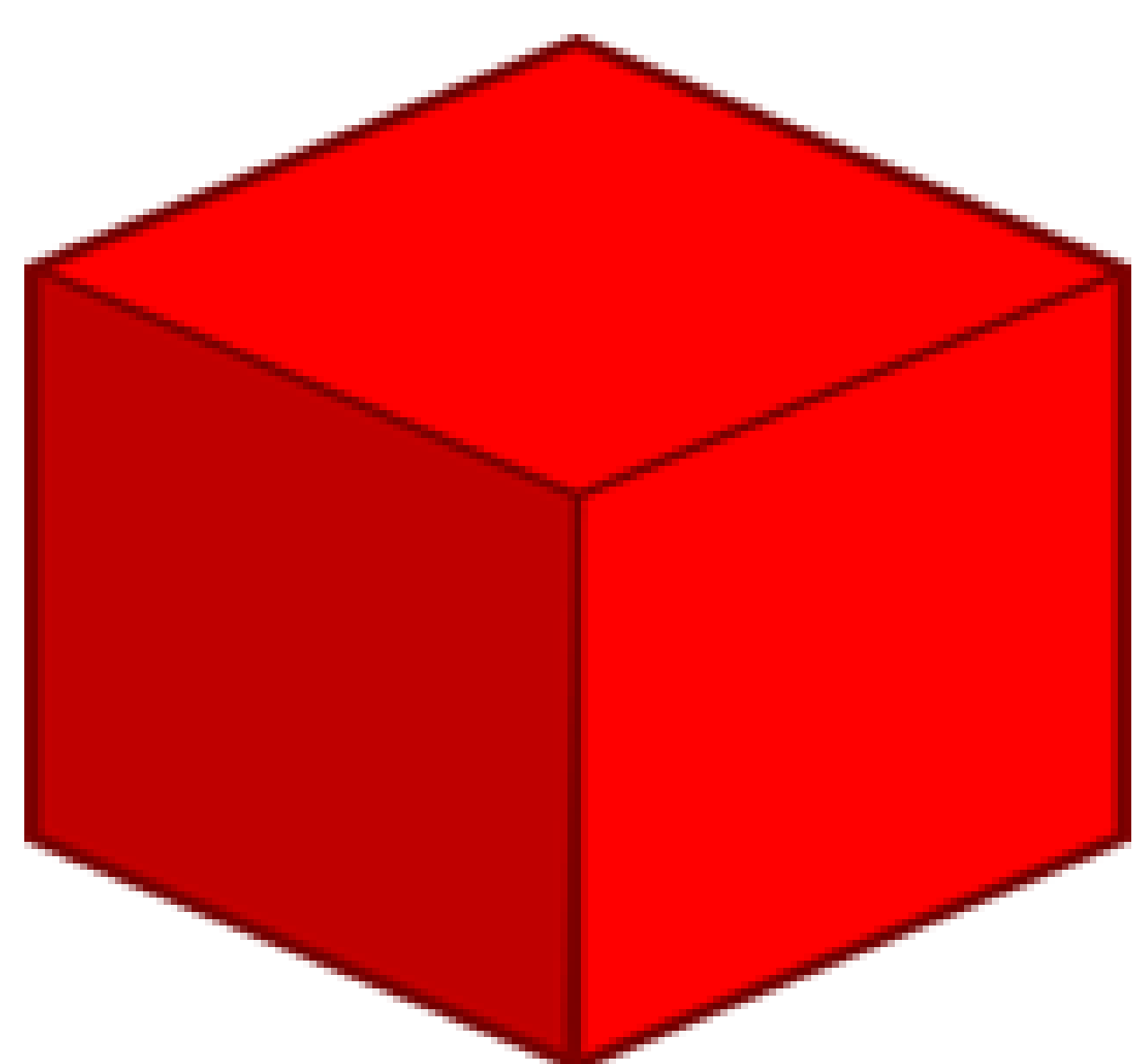
Cube
